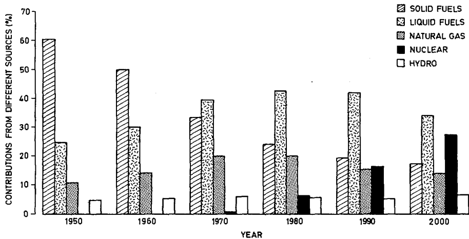
FIG. 1. 7. Contributions of various primary energy sources to electricity generated to the year 2000. (With reference to the 1973 forecast.)
